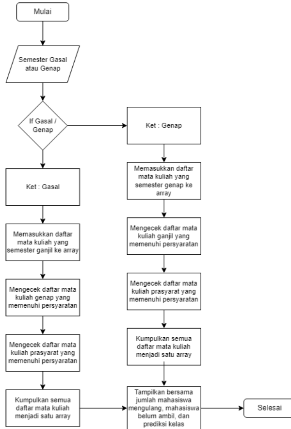
Gambar 1. Flowchart Sistem
